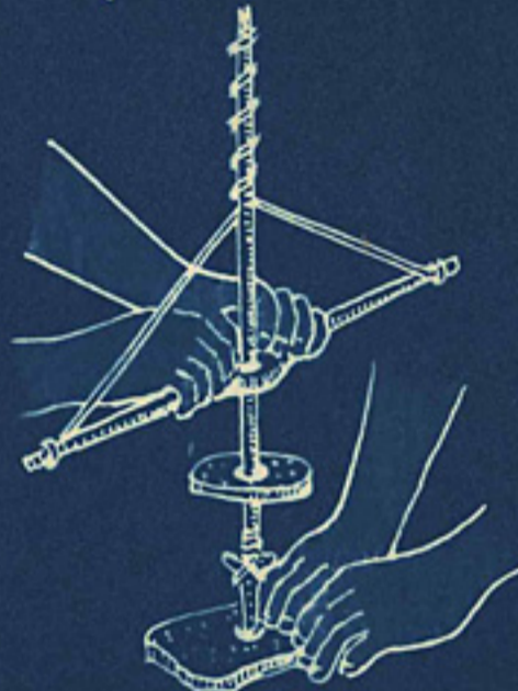
STONE DRILL FIXED ON SHAFT AND HOLE IN STONE MADE WITH THIS DRILL
